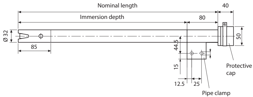
Pipe clamp
