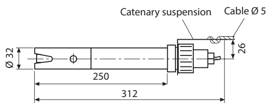
Catenary suspension
