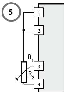
Potentiometer: 4-wire
