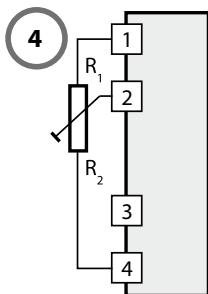
Potentiometer: 3-wire
